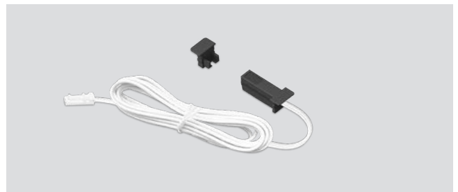
Proximity switch ON-OFF / DIMMER (10-100%) - Range: 3-6cm MAX: 1,5A - 36W (Lamp up to 3600mm)
